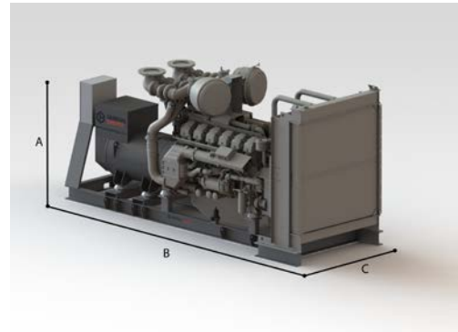
A= 2935 mm B= 5242 mm C= 2246 mm
